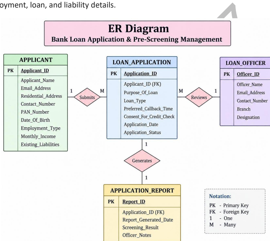
Fig. 4. Entity-Relationship Diagram for the Bank Loan Application Data Model
